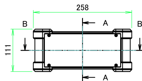
A view
