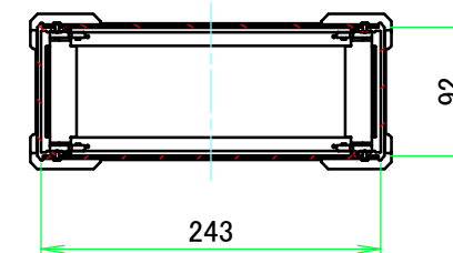
C-C (1:6)
