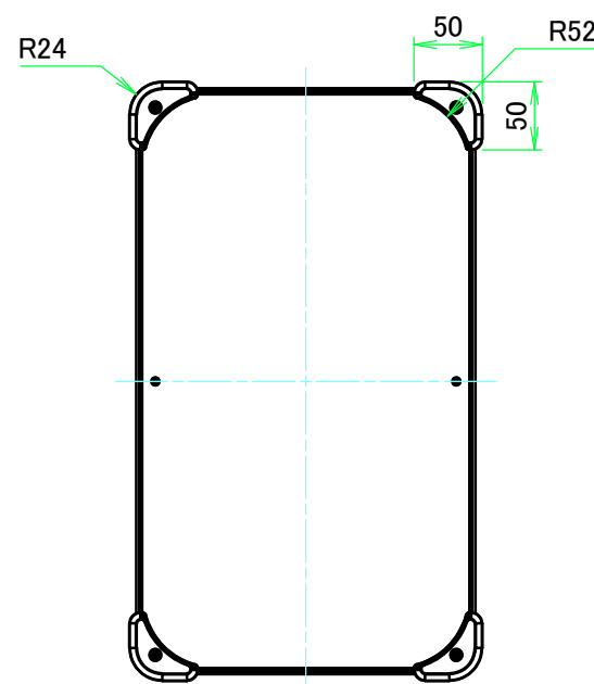
F view
