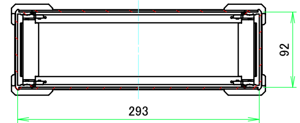
C-C (1:4.5)
