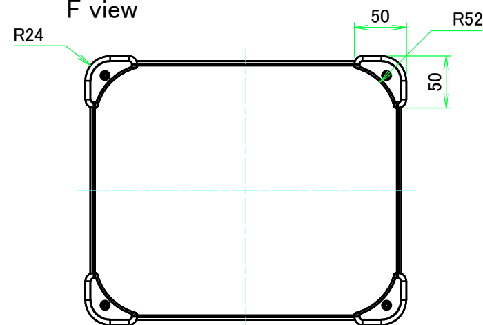
F view
