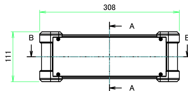
A view
