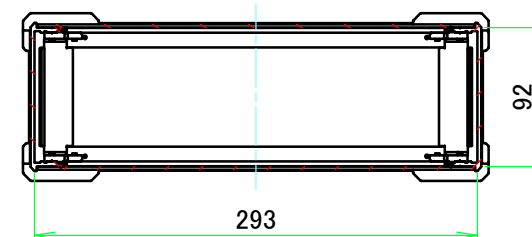
C-C (1:5)
