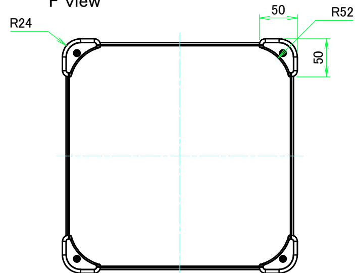
F view
