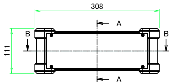
A view
