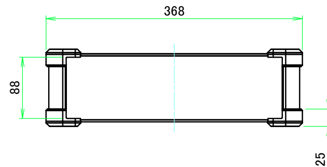
C view
