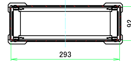
C-C (1:6)
