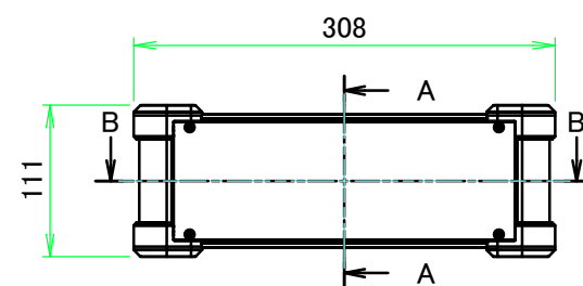
A view
