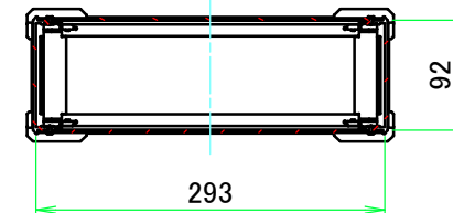
C-C (1:7)
