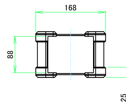
C view
