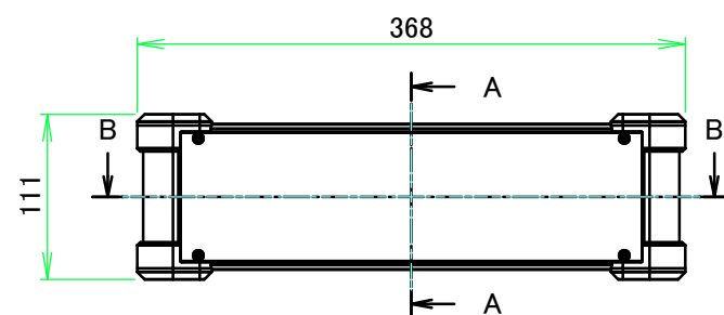
A view
