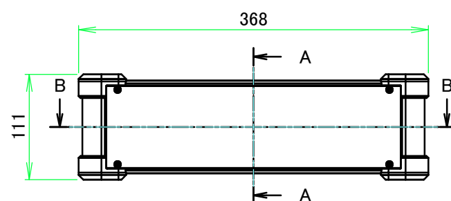
A view
