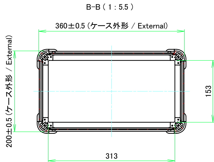
D view
