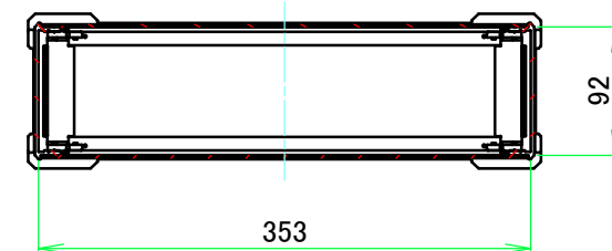
C-C (1:6)
