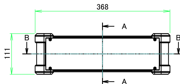
A view
