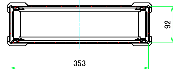
C-C (1:6)
