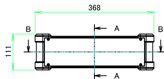
A view
