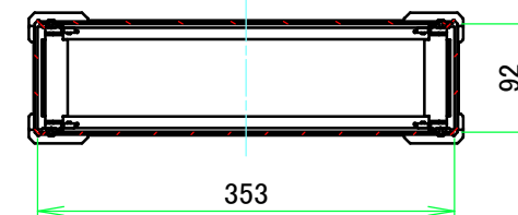
C-C (1:7)
