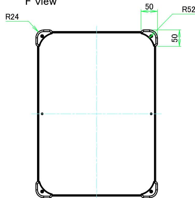
F view
