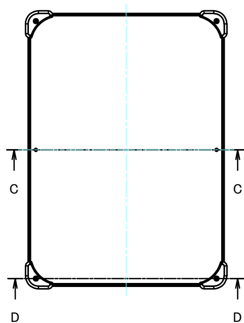
E view
