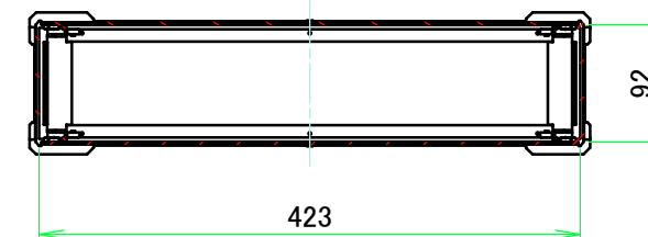
C-C (1:6.5)
