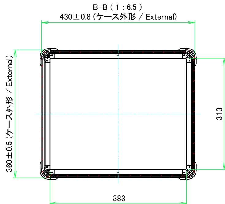
D view
