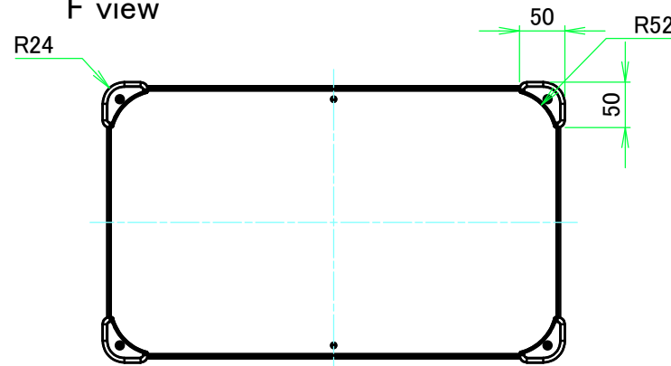
F view
