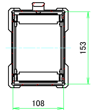
C-C (1:5)
