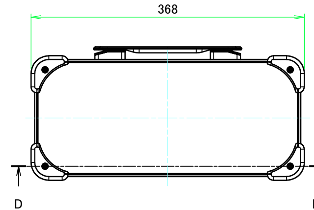
E view
