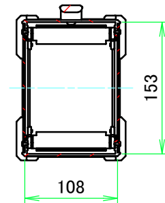
C-C (1:6)
