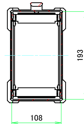
C-C (1:5)
