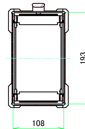
C-C (1:5)
