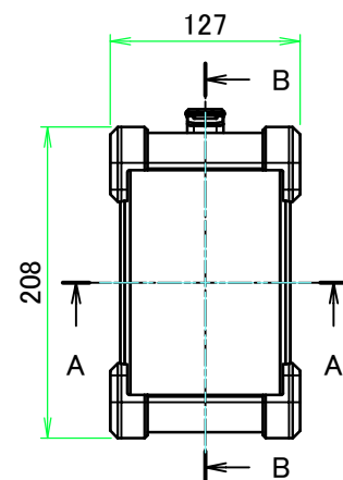
A view
