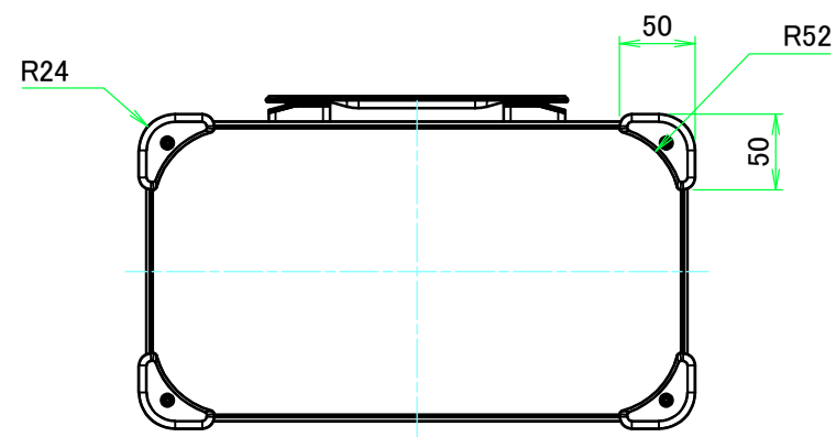
F view
