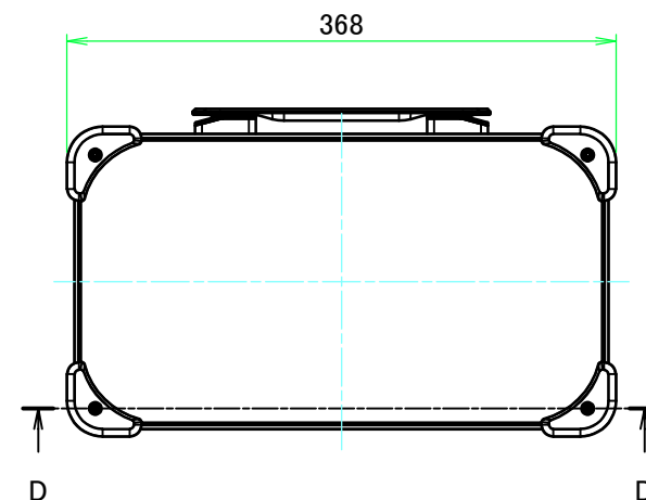
E view
