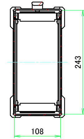
C-C (1:5.5)
