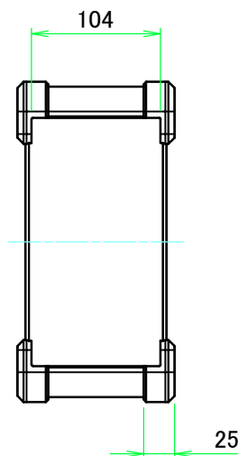
D view
