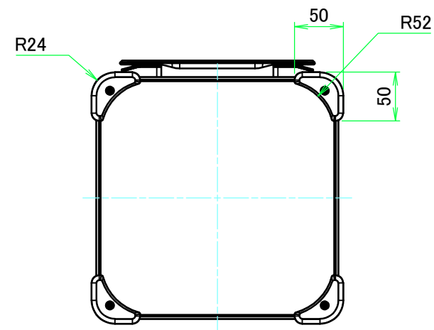
F view
