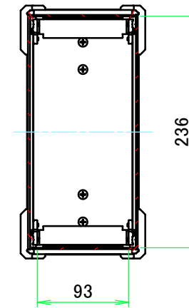
A-A (1:5.5)
