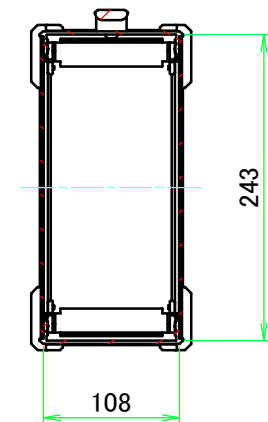
C-C (1:6)
