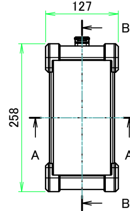
A view
