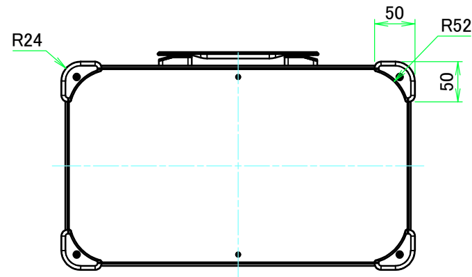
F view
