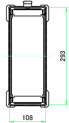
B view
