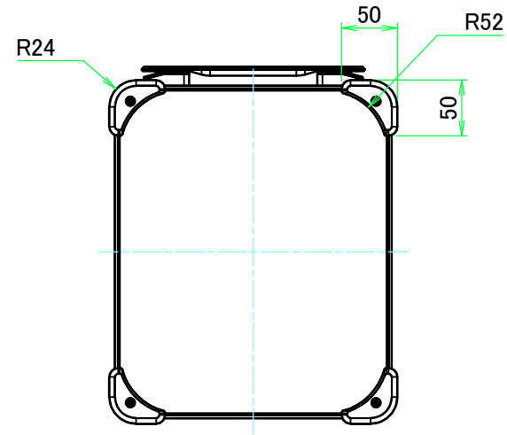
F view
