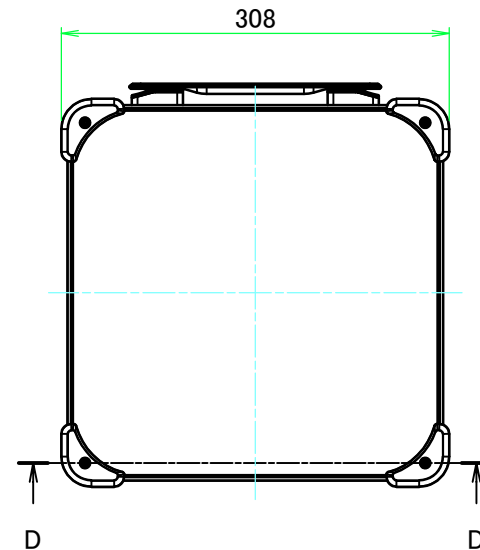
E view
