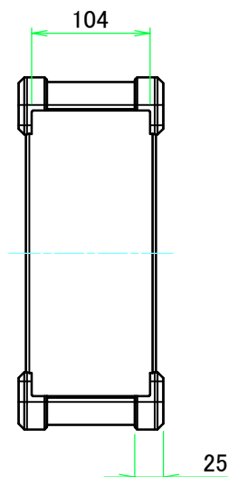
D view
