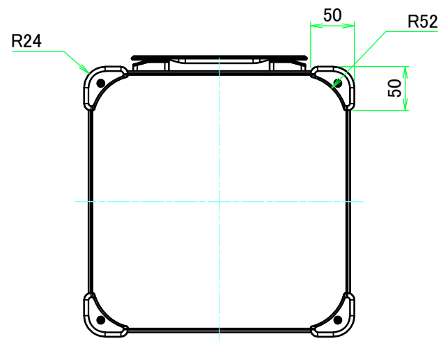
F view
