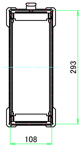
B view
