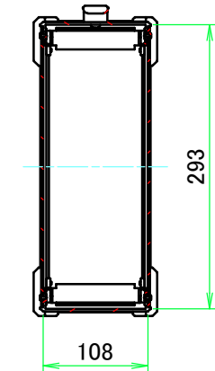
C-C (1:7)
