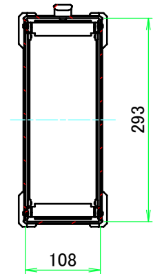
C-C (1:7.5)
