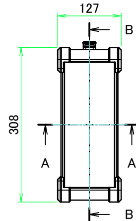
A view
