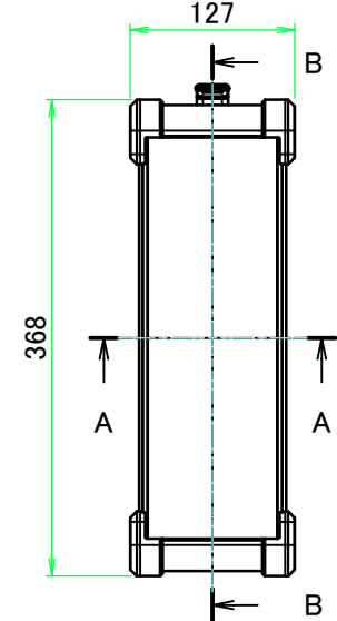
A view
