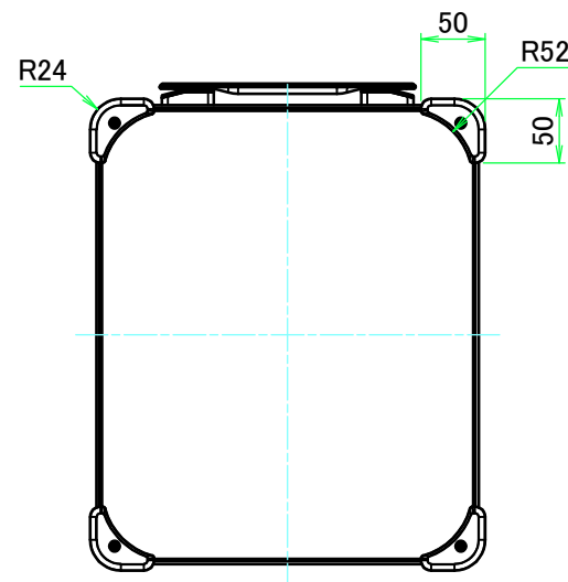
F view
