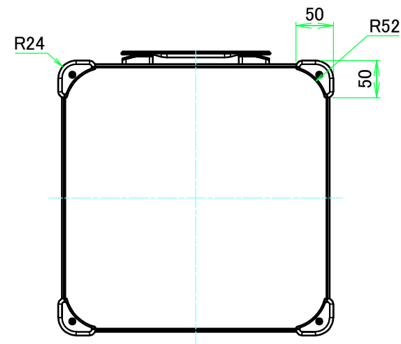
F view
