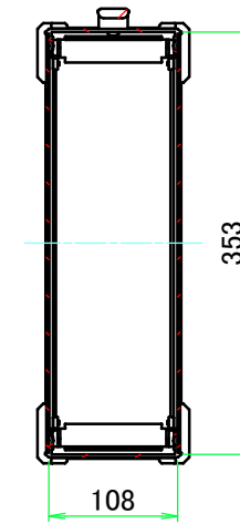
C-C (1:7)
