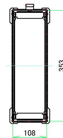
C-C (1:7)
