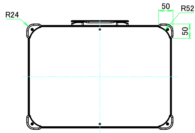
F view
