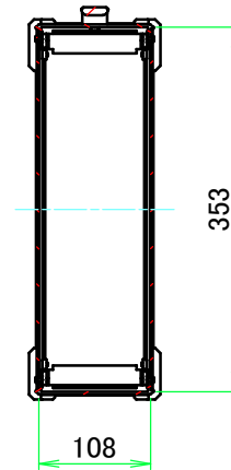
C-C (1:8)
