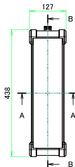
A view
