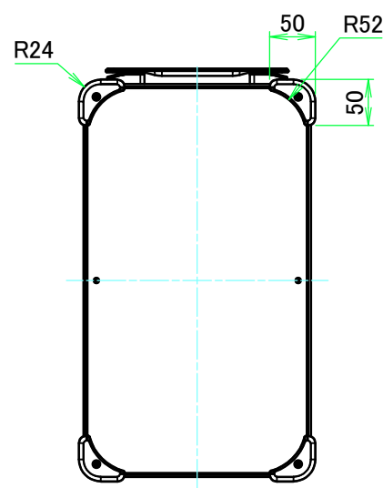
F view
