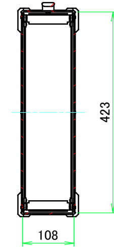
C-C (1:8)
