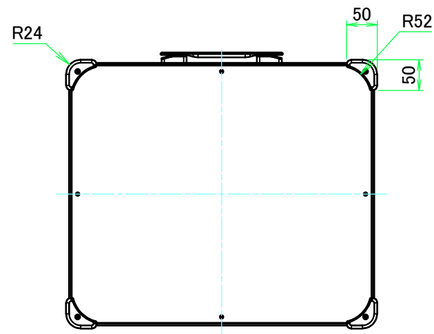
F view
