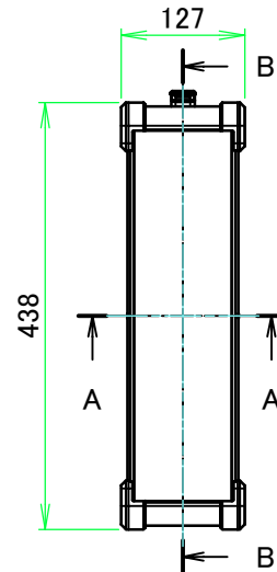
A view
