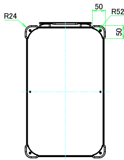
F view
