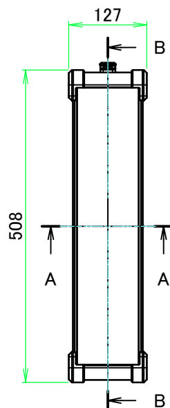
A view
