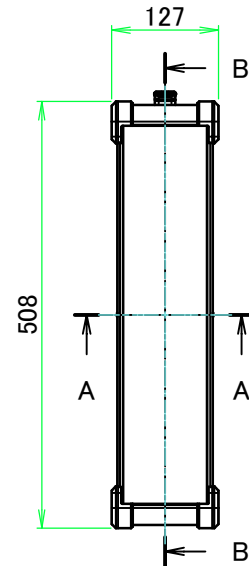
A view
