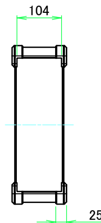
D view
