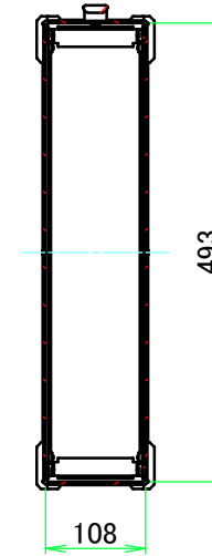
B view
