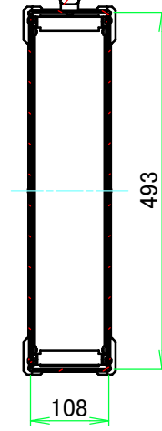
B view
