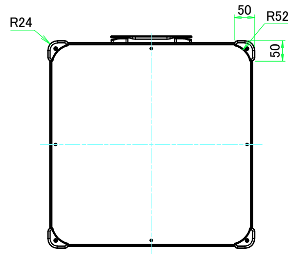
F view
