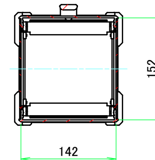
C-C (1:5.5)
