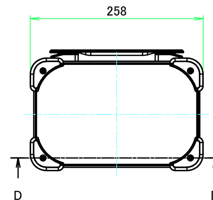
E view
