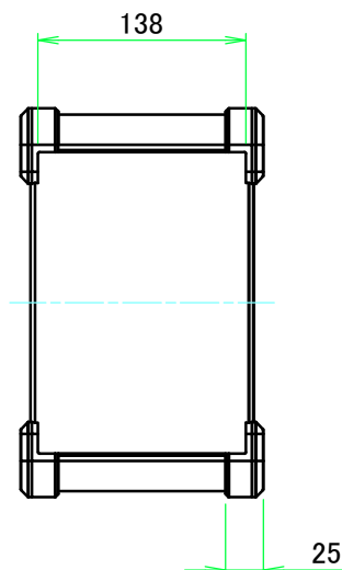
D view
