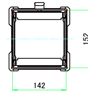
C-C (1:6)
