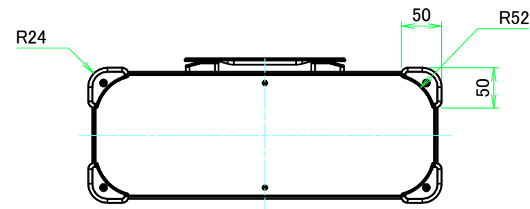
F view
