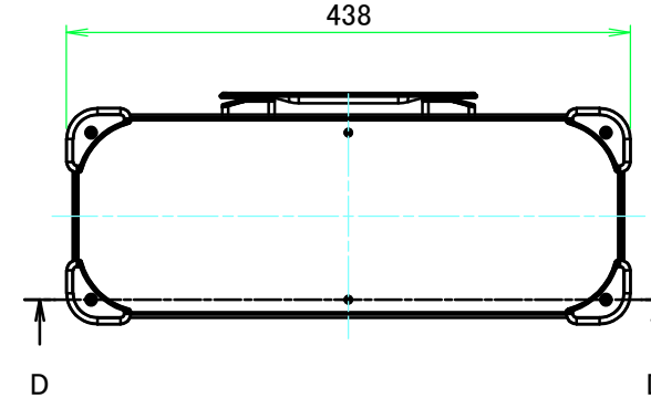
E view
