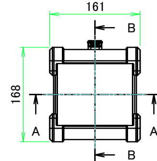
A view
