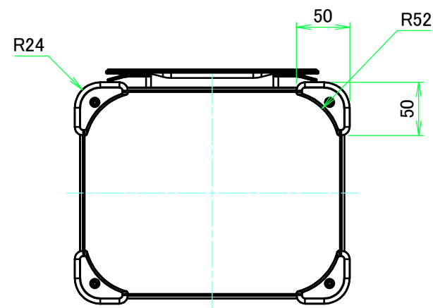
F view
