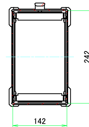
C-C (1:6)
