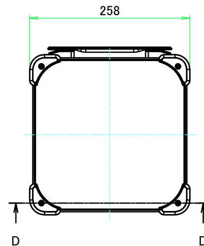
E view
