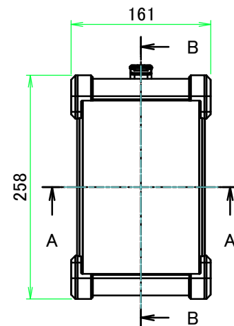
A view
