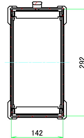
C-C (1:6)
