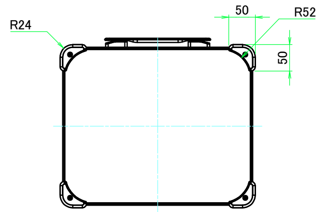
F view
