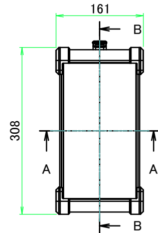
A view
