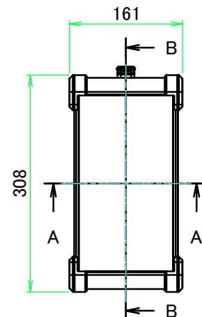
A view
