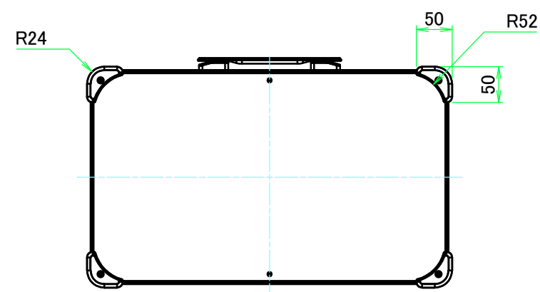
F view
