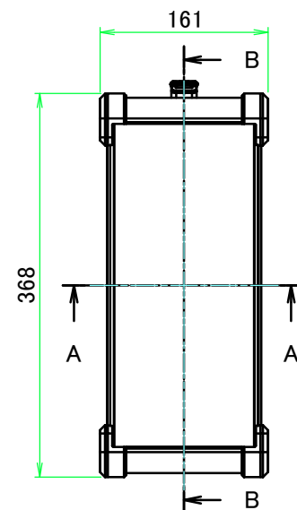
A view
