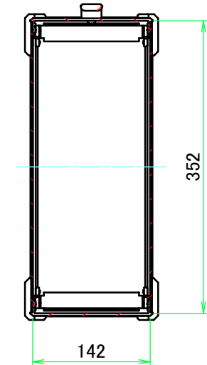
B view
