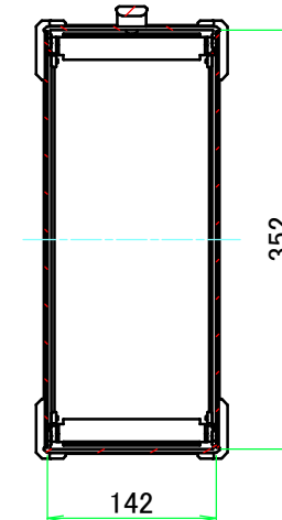
C-C (1:7)
