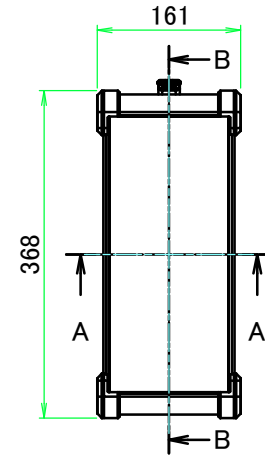
A view
