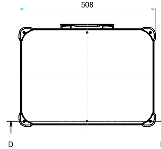
E view
