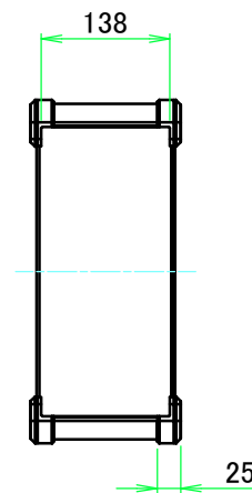
D view
