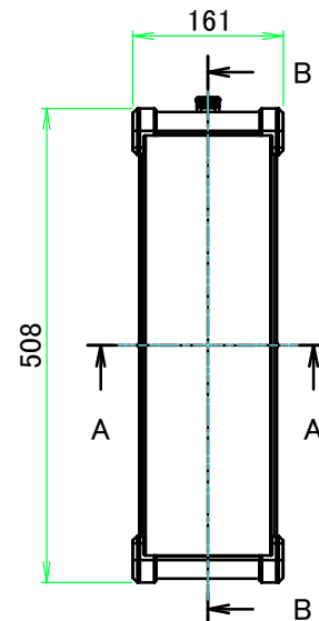
A view
