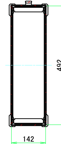
B view
