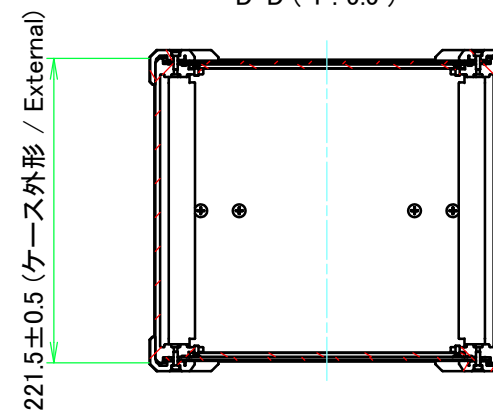
D-D (1:5.5)
