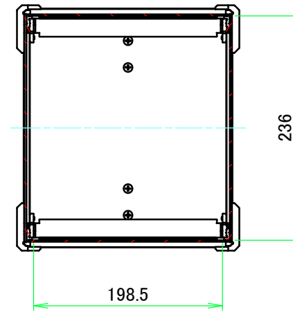
A-A (1:5.5)
