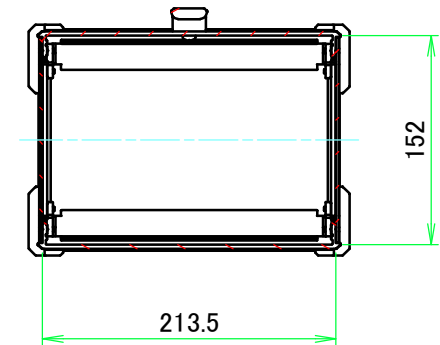
C-C (1:5.5)
